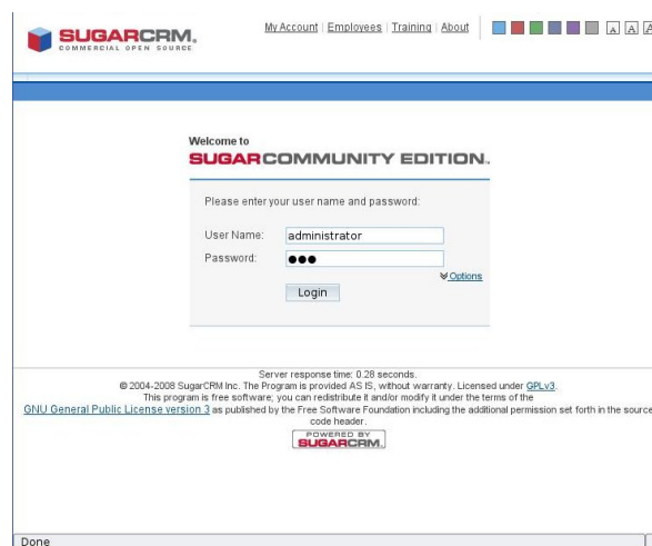
Figure 1: Login interface
