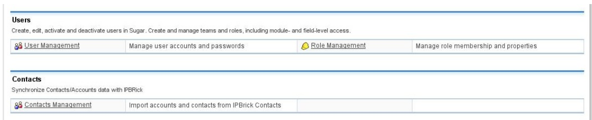
Figure 2: Administration interface
